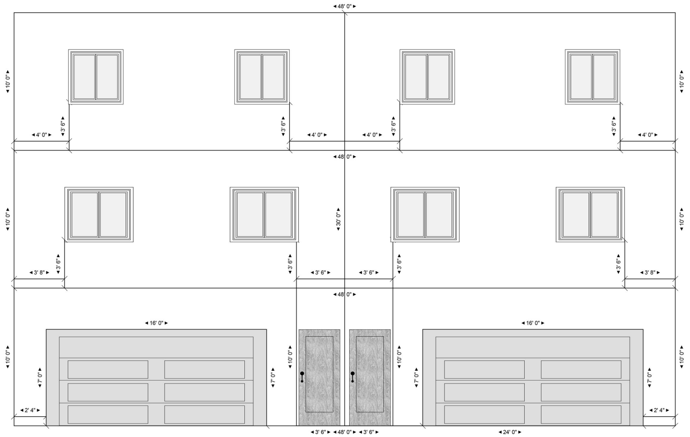
Marengo St front elevation
