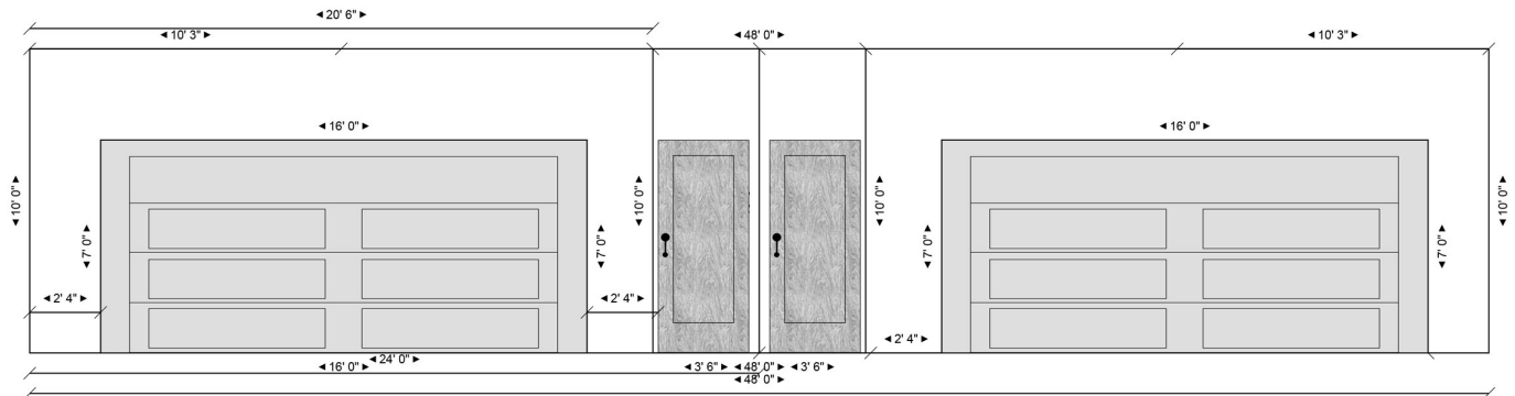
N. Alma St front elevation (street level, 3rd flr)
