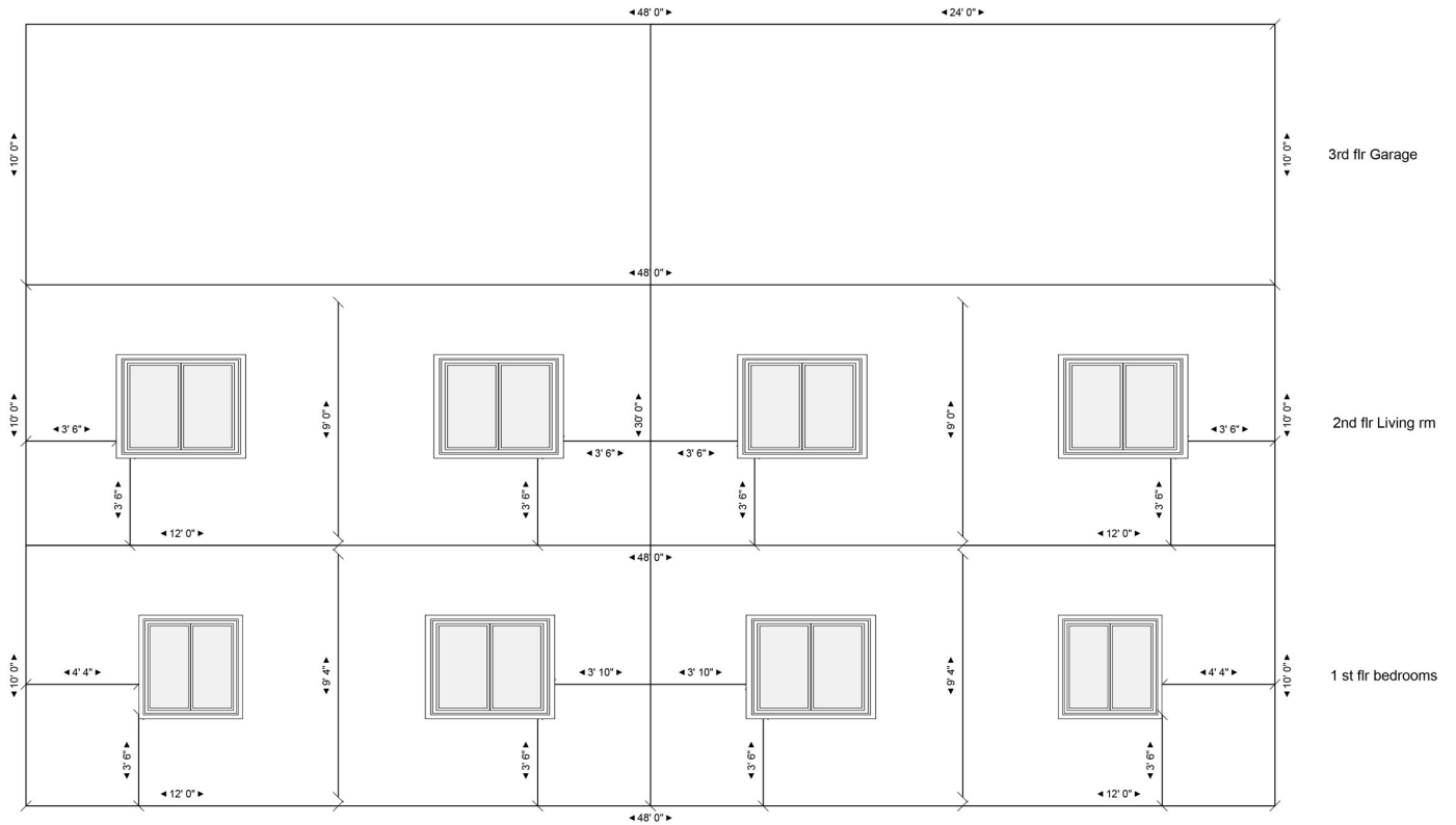
N. Alma ST rear view elevation
